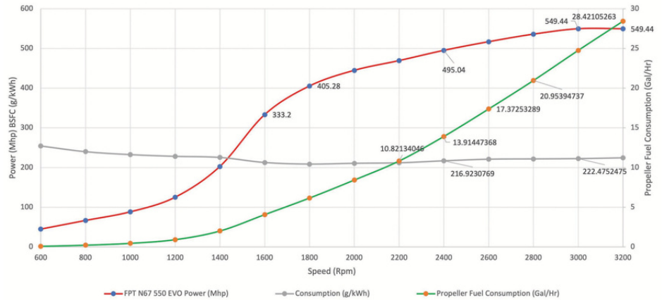
FPT N67 550 EVO Performance
