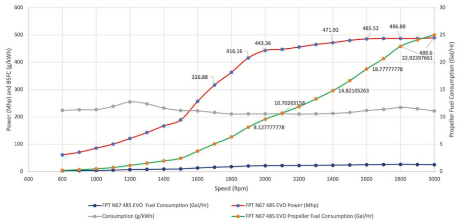
FPT N67 485 EVO Performance B Rating
