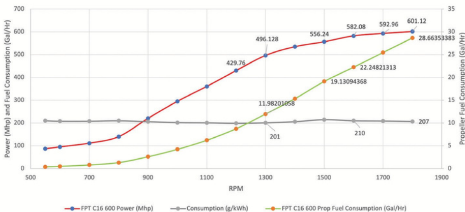
FPT C16 600 Performance Curve
